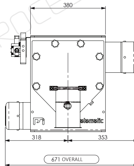
WITHOUT FORCED VENTILATION FOR SCREW FEEDER ENGINE
